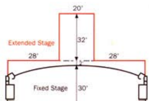
Catwalk Stage Extension
