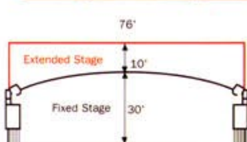
Standard Stage Extension
