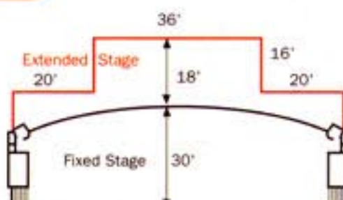
T-Shape Stage Extension
